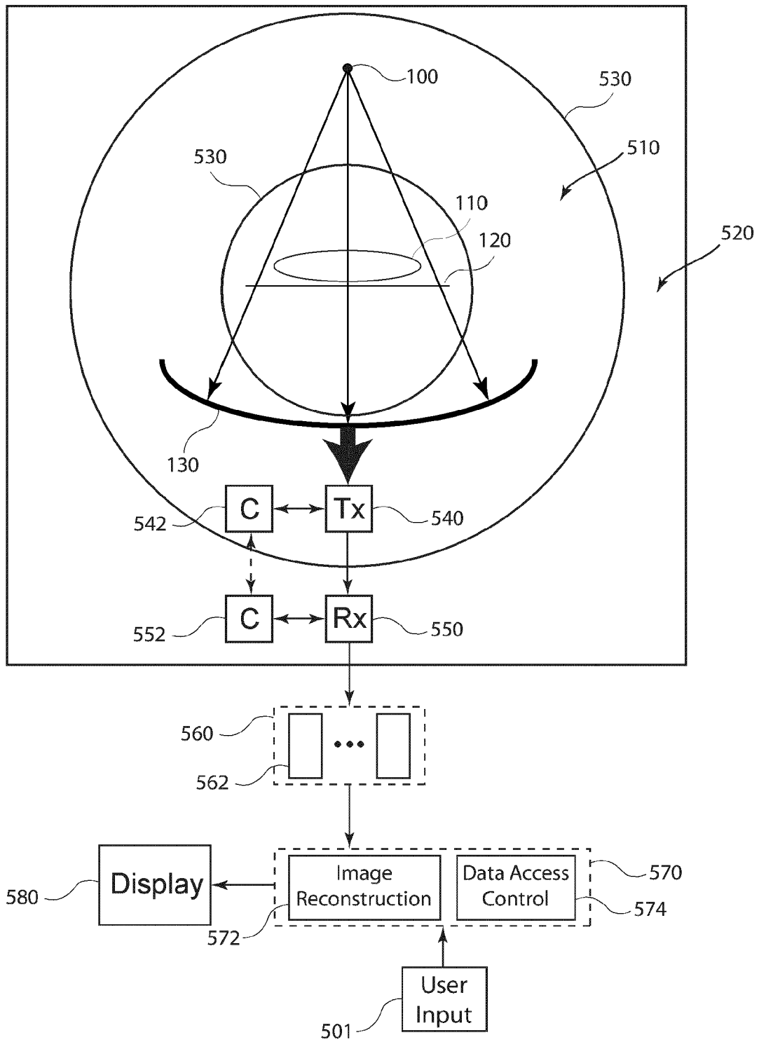
Figure 2 Prior Art
